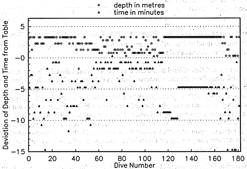
Figure 3. Choice of table depth and time in 181 SurD dives in the NDC data base, 1989 Sept. Dives with actual time shorter than table time are shown below the zero line, while dive depths shallower than table depth are shown above this line.
