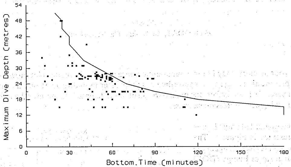
Figure 2. NDC Data Base: Plot of 181 SurD dives in September 1989. The continuous line represents the DOE bottom time limits.
